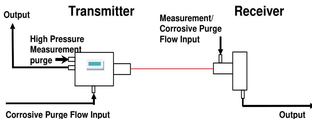
Figure 3-2: Purging of the transmitter and receiver units
