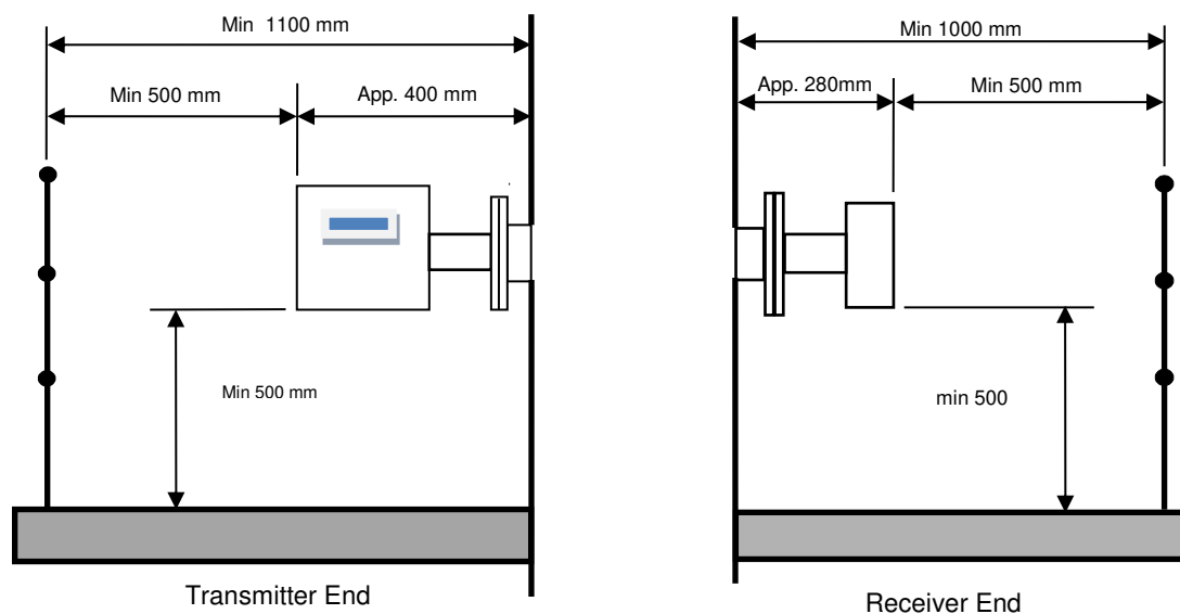
Figure 2-1: Transmitter and receiver installation tolerances
