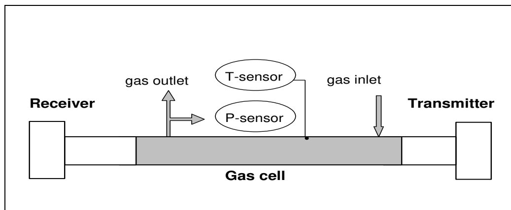
Figure 5-1: Calibration cell with monitor connected
