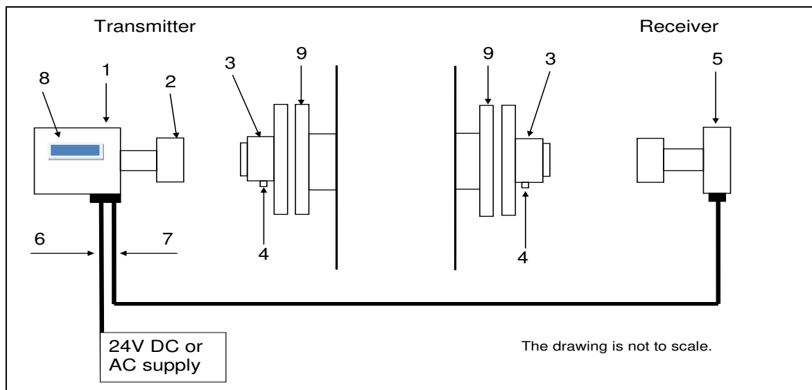
Figure 3-1: SERVOTOUGH Laser Monitor units and their main components
