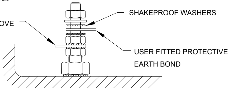
b) Method of fixing protective earth connection
