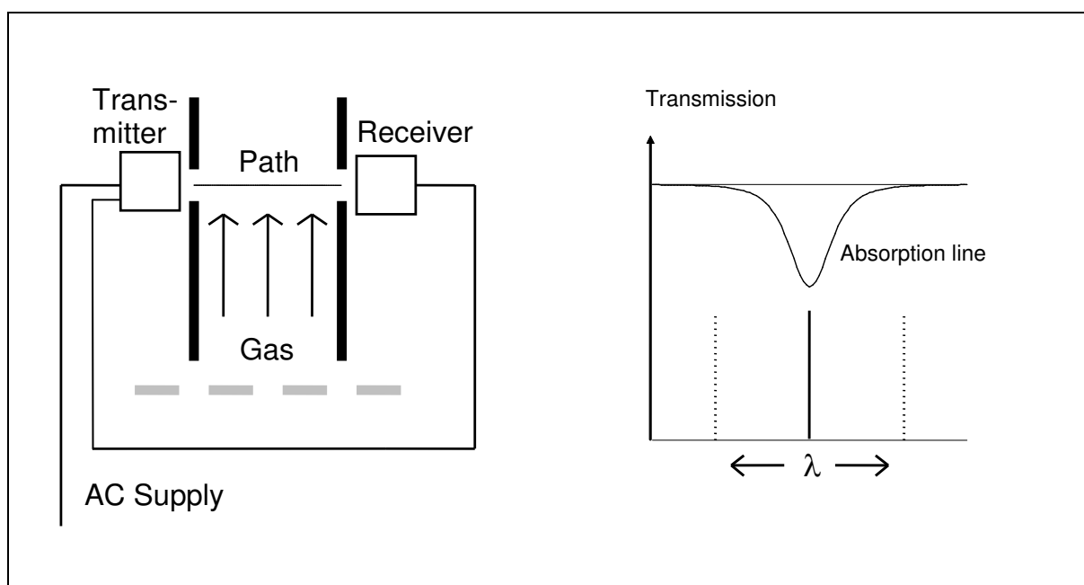
Figure 1-1: Measuring Principle SERVOTOUGH Laser Monitor
