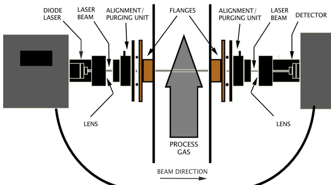
Figure 1-2: General view of SERVOTOUGH Laser Monitor
